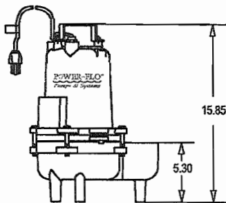
PFS411 & PFS421 without float
