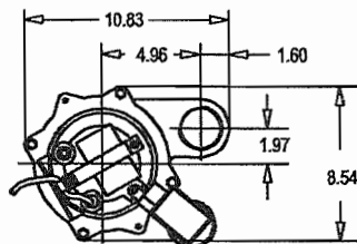
PFS411VF vertical level control with piggy-back plug
