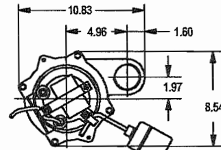
PFS411A with automatic float
