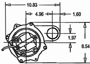
PFS411 & PFS421 without float
